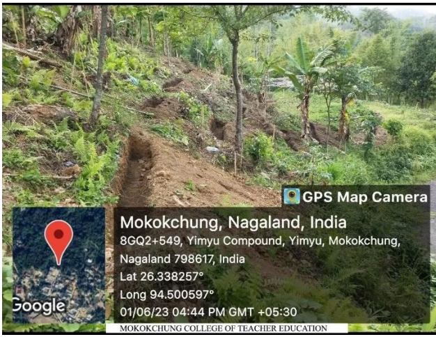
Fig: Contour trenching for ground water (JSA-CTR 2023)
